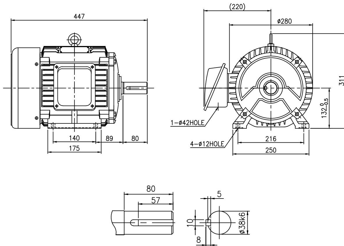
SHAFT EXTENSION
