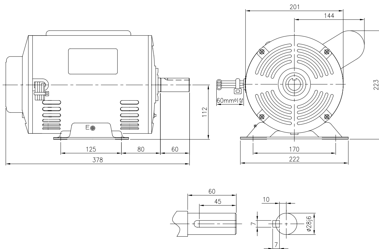
SHAFT EXTENSION
