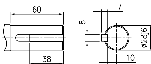
SHAFT EXTENSION
